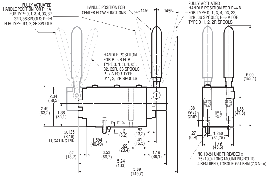
6100 Series, Lever Operated Models
