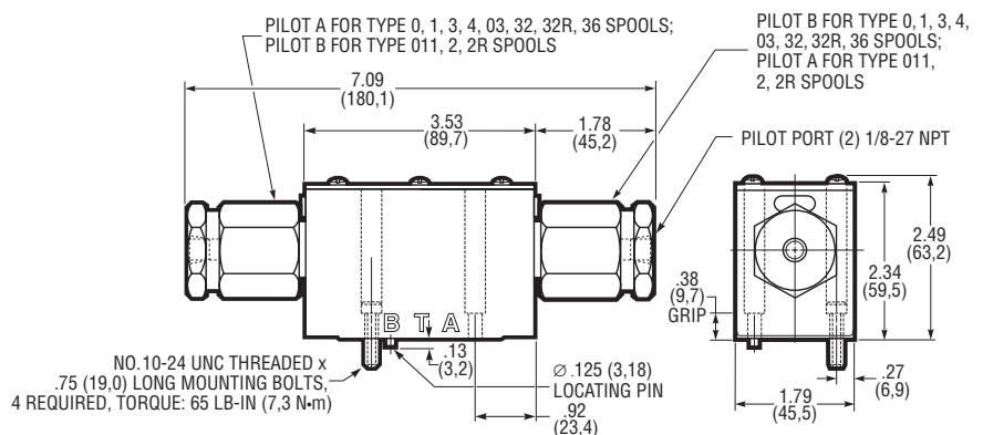
6900 Series, Double Air Piloted Models
