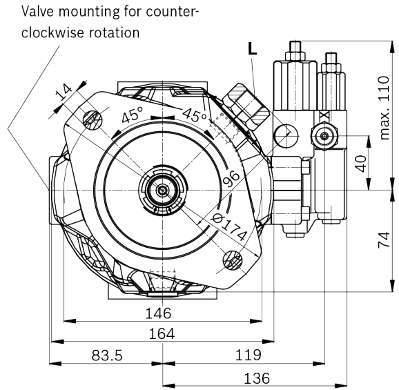
Detail W
