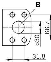
Detail V
