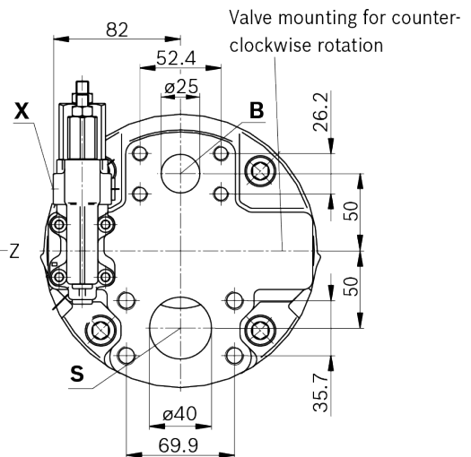
View Z
