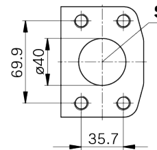
View Z
