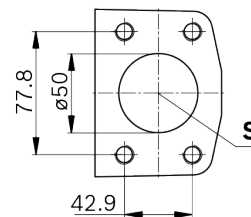
Detail W
