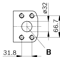
Detail V
