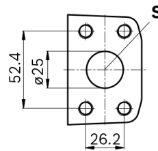
Detail W
