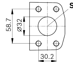
View Z
