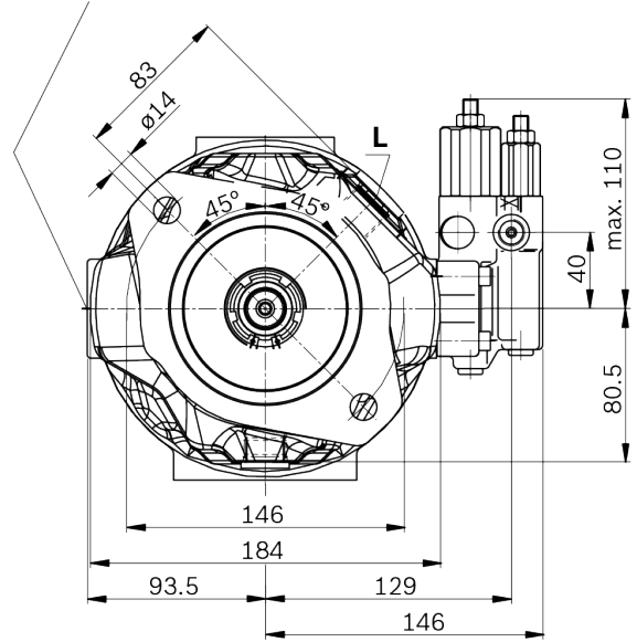
Detail W
