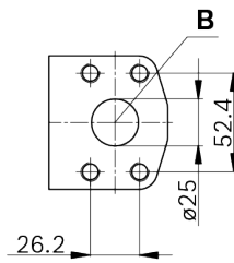
Detail V
