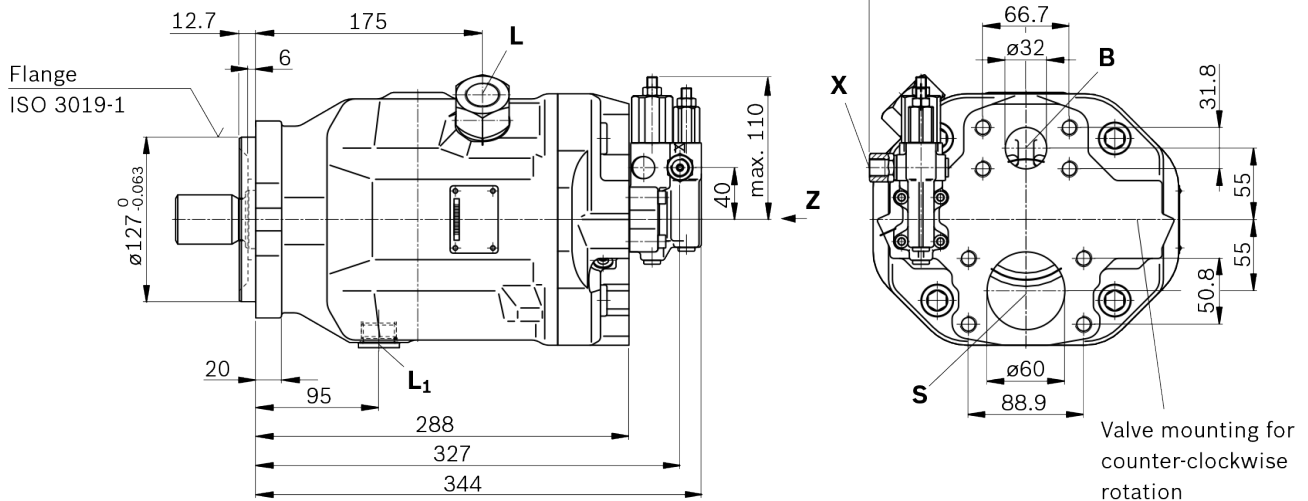
View Z
