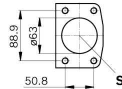
View Z
