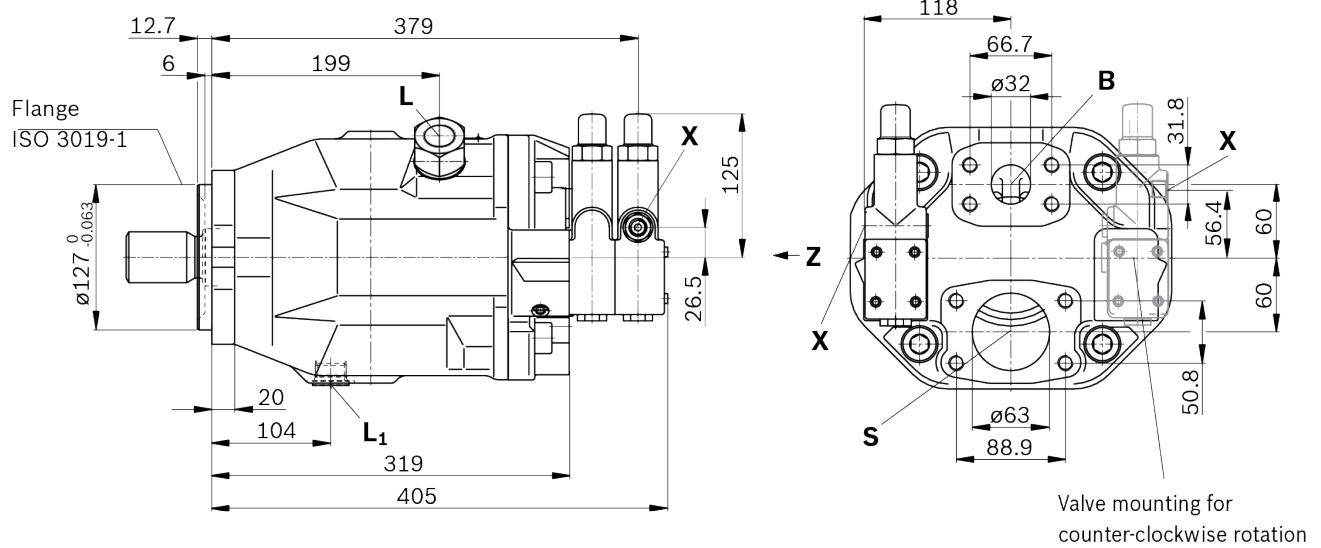
View Z
