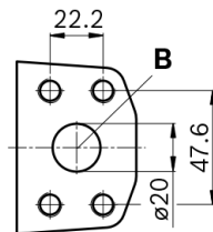
Detail V
